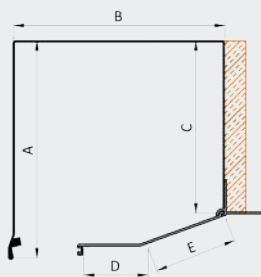
BENDED ROLLER SHUTTER BOX 20° it can be plastered, with extruded moun- ting panel
