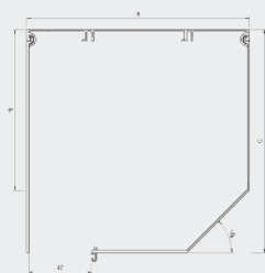
EXTRUDED ROLLER SHUTTER BOX 45°/20°
