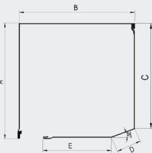
BENDED ROLLER SHUTTER BOX 20°
