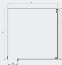
BENDED ROLLER SHUTTER BOX 90° it can be plastered, with extruded moun- ting panel
